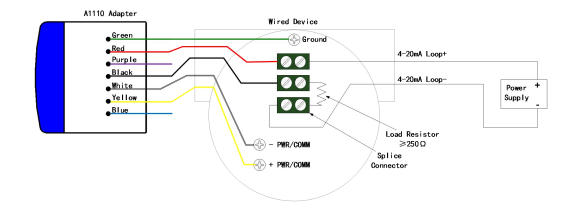
Figure 3-3 Two-wire Device Wiring Diagram When Loop Powered
