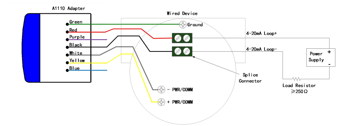
Figure 3-4 Two-wire Device Wiring Diagram When Loop Powered (with resistor)
