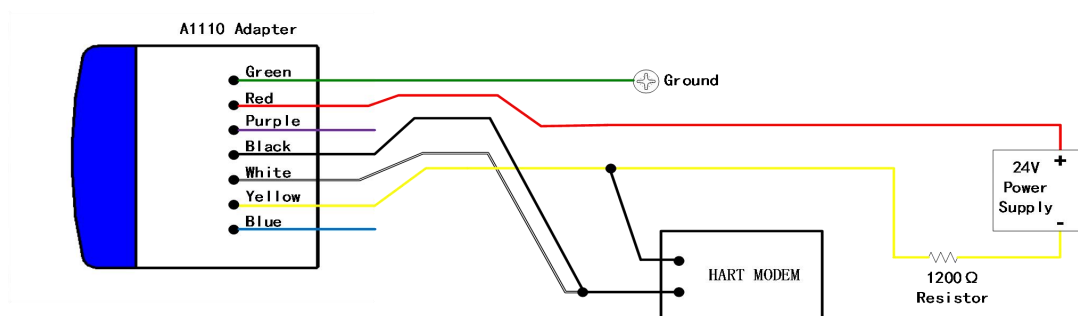
Figure 2-2 A1110 configuration connection mode
