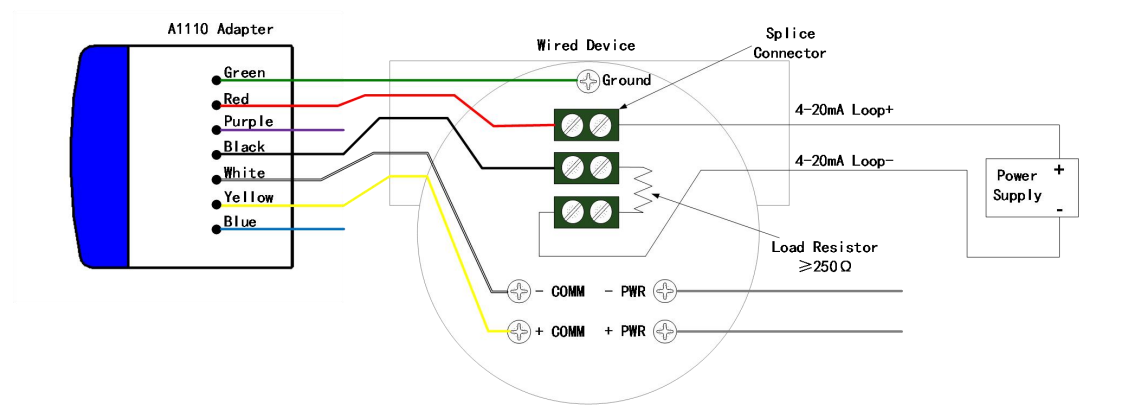
Figure3-5 Four-wire Device Wiring Diagram When Loop Powered
