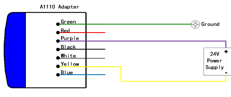
Figure 3-2 Wiring Diagram of A1110 as Repeater
