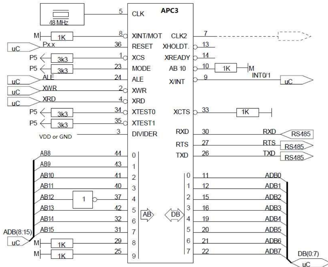
Figure 6.4 80C32 Application
