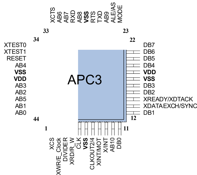
Figure 2.1 Definition of pin outgoing line
