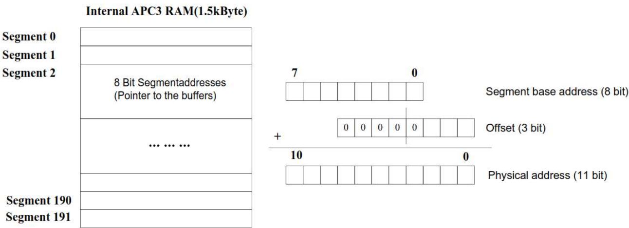
Figure 3.1 Schematic Diagram of APC3 Memory RAM Segmentation
