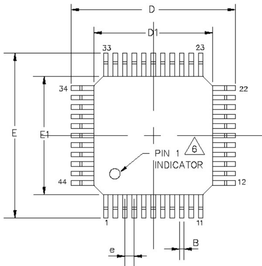
Figure 7.1 Package Drawing
