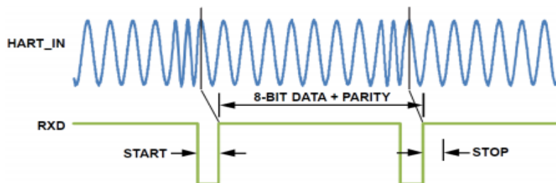
Figure 10 HT5700 Demodulator Waveform (Preamble Message 0xFF)
