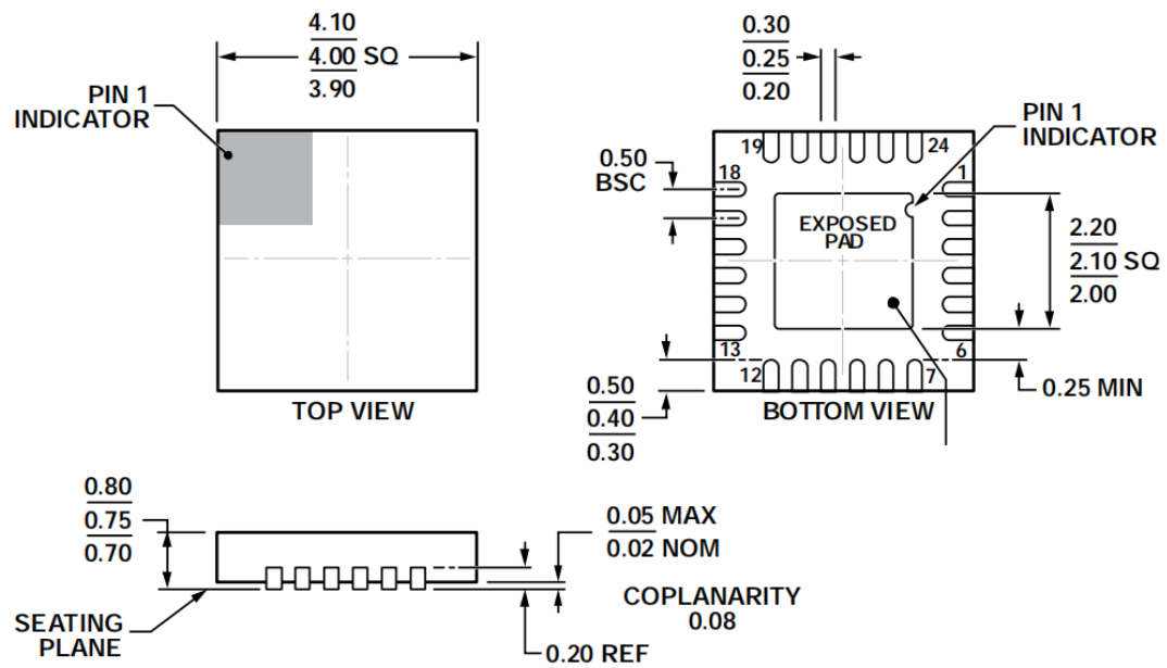
Figure 19 Package Description
