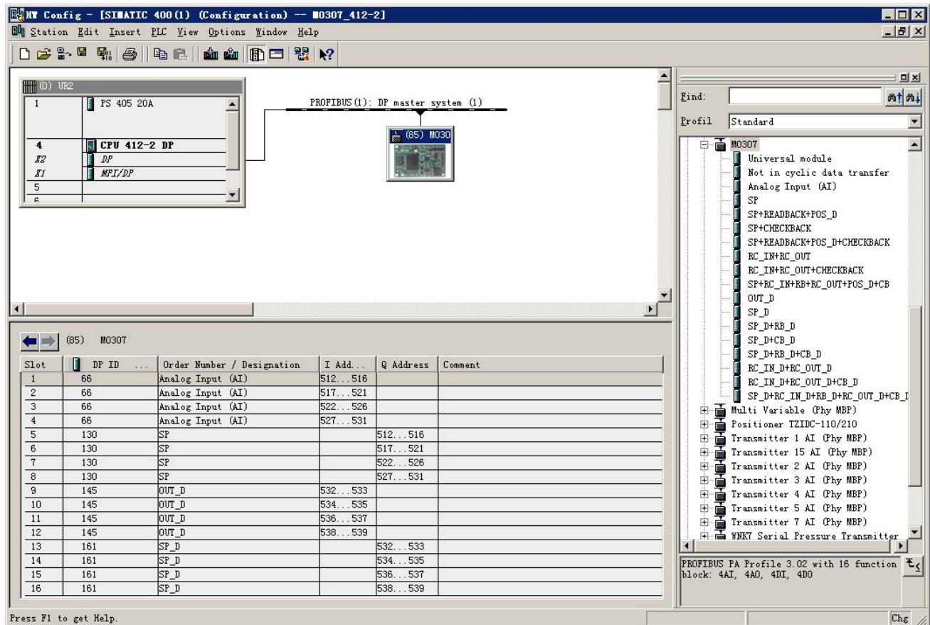
Figure 4.7 Device Configuration
