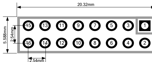
Figure 2.2 User interface pin definition and dimensions
