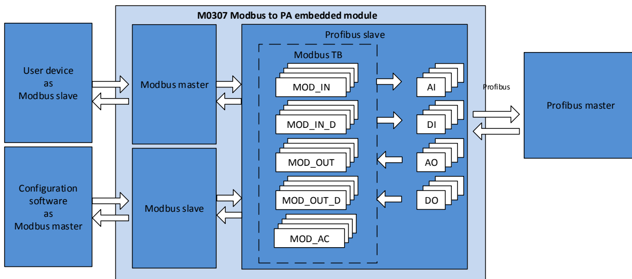
Figure 3.2 working principle
