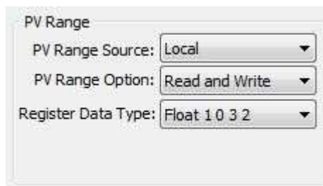
Figure 3.4 PV Range Operation
