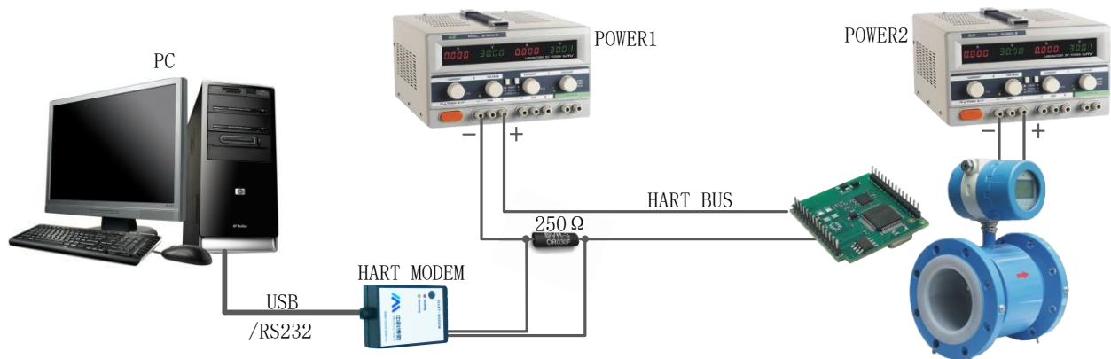
Figure 1.2 Configuration HART module wiring diagram
