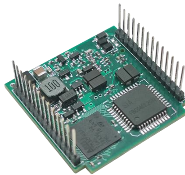
Figure 1.1 MC0313 Modbus to FF Embedded core module
