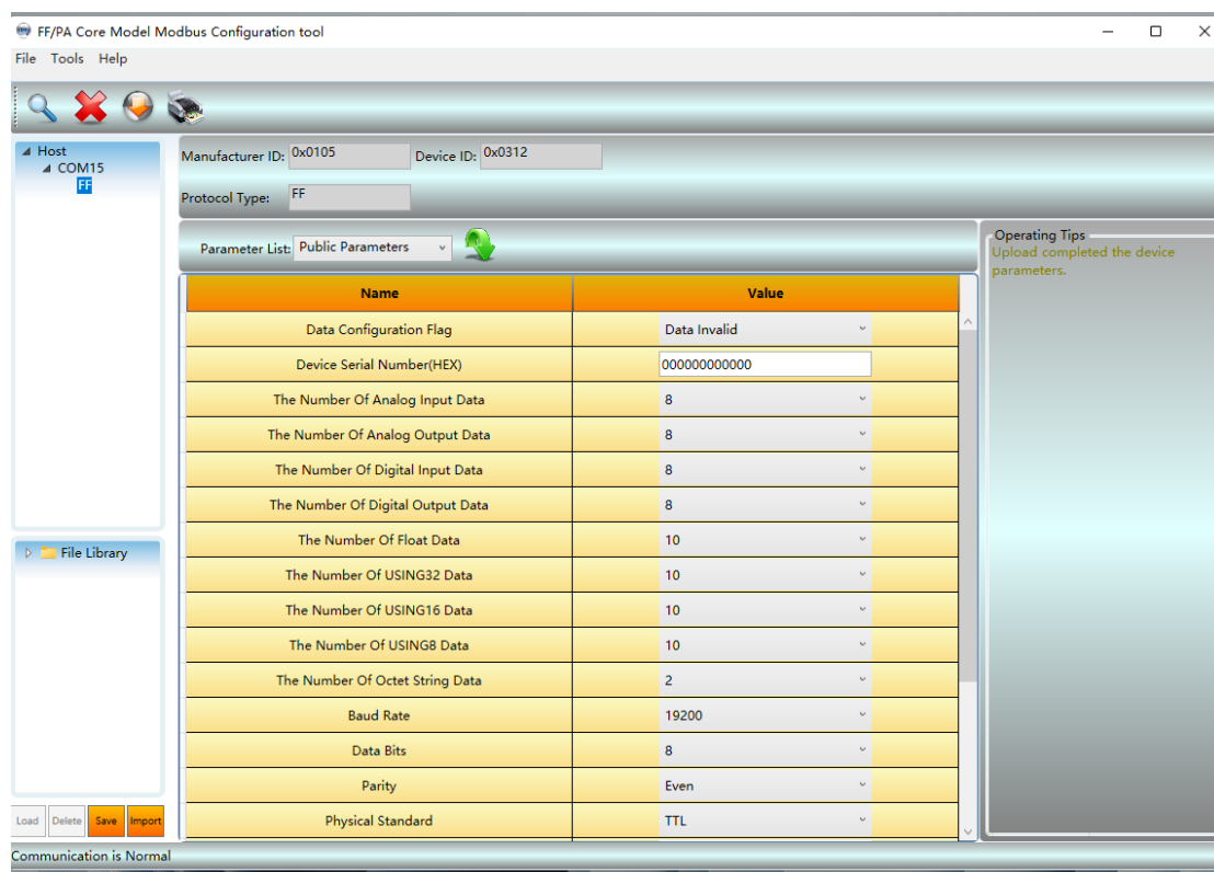
Figure 4.6 Scanning equipment
