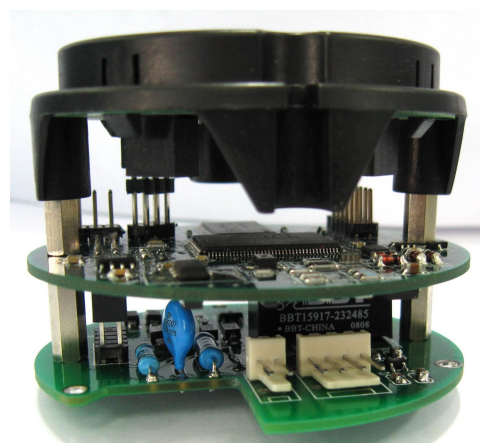
A FF/PA Board Set
