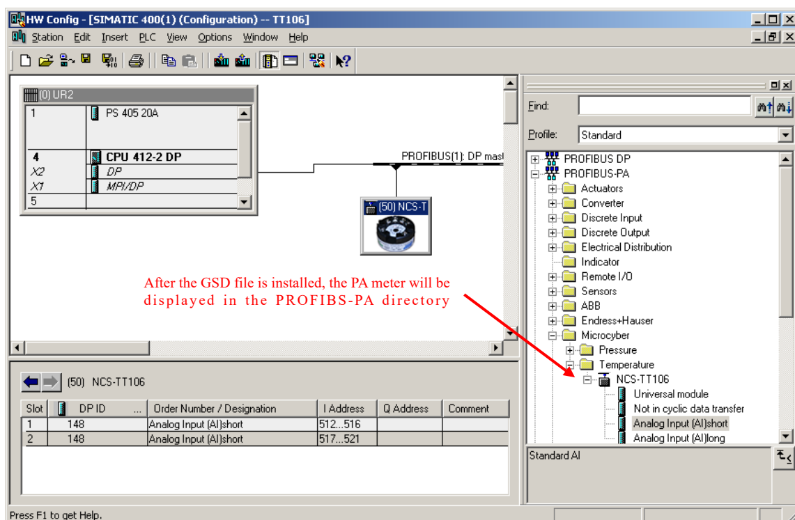
Figure 3.6 Drag the PA device to the PROFIBUS DP bus
