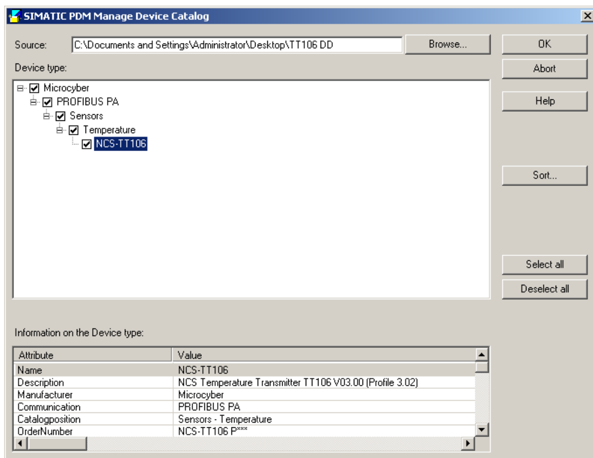
Figure 3.8 Select device type
