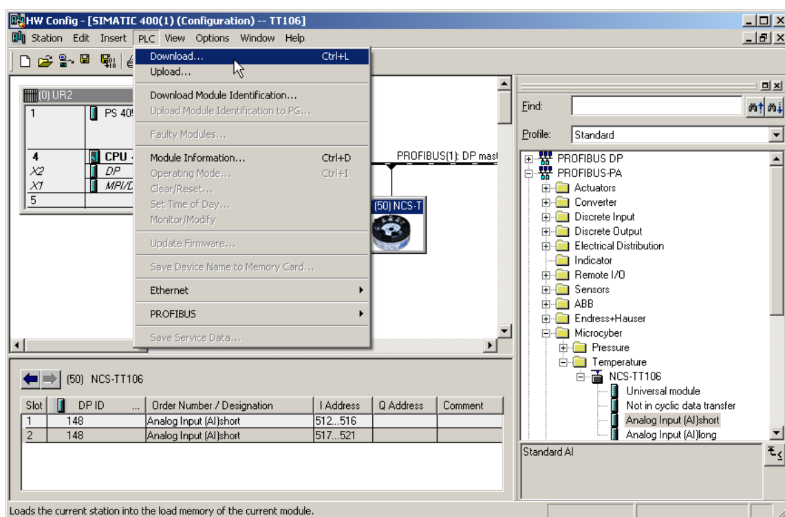
Figure 3.7 Download configuration information to PLC
