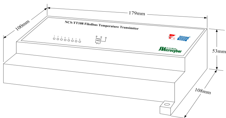
Figure 3.2 Dimensions
