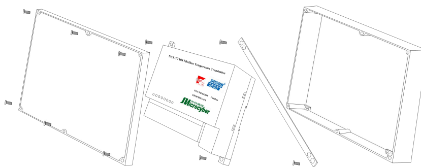
Figure 2.4 Mounted in outdoor box
