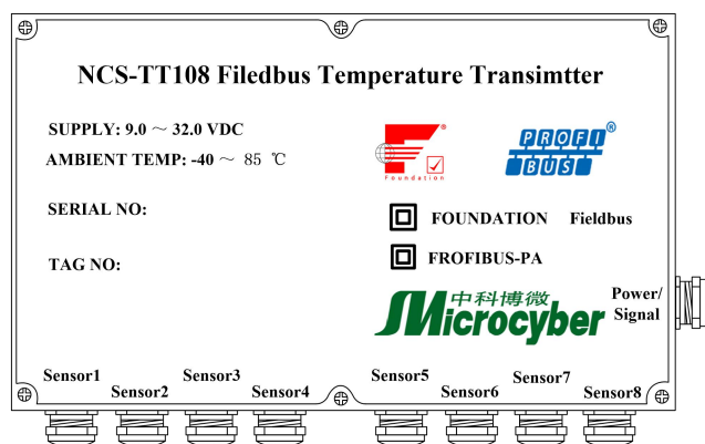
Figure 2.3 Outdoor case
