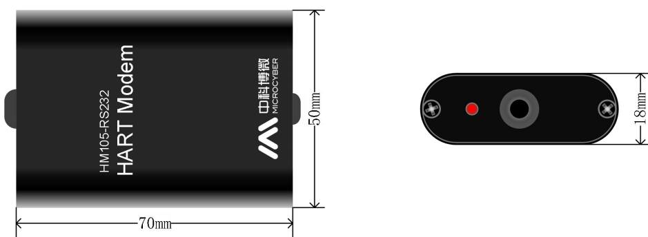
Figure 2 Dimension (70*50*18, unit mm)
