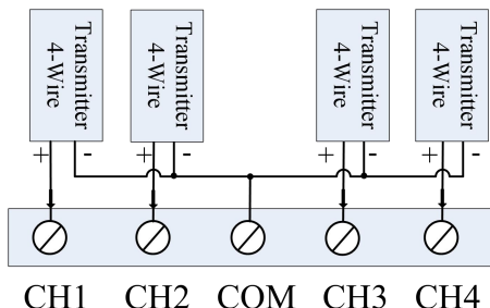
Figure 2.7 Wiring of NCS-IF105 Converter (4- Wire)
