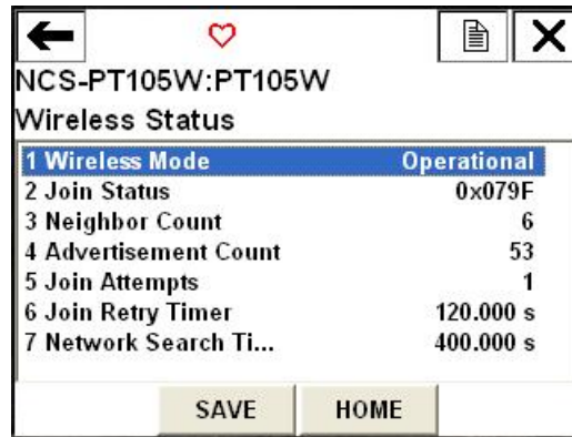
Figure 4.10 475 communicator WirelessHART
