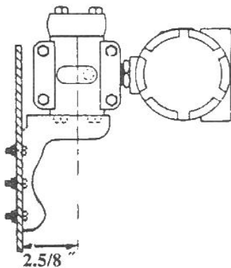
Figure2.1 B2 Flat bracket tube installation plate installation
