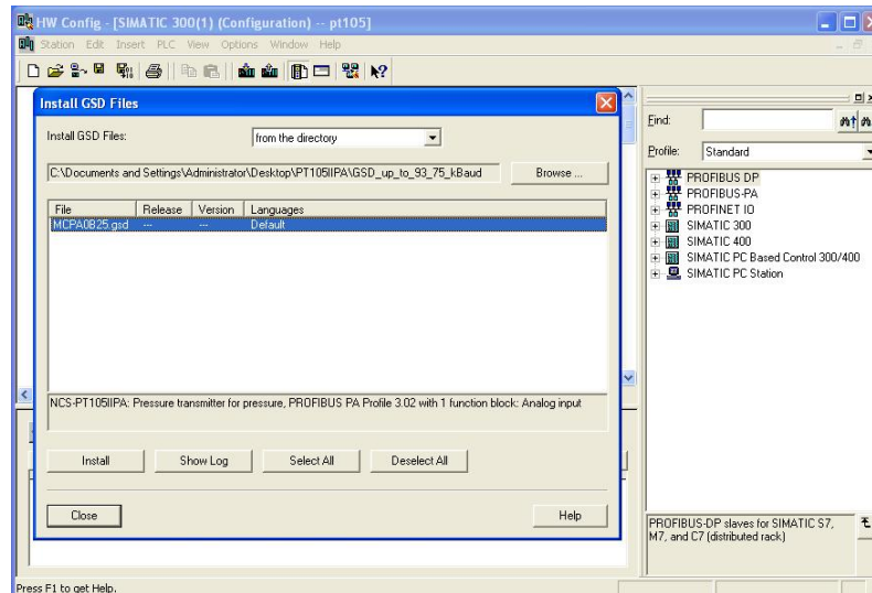
Figure 7.5 Installing the GSD file
