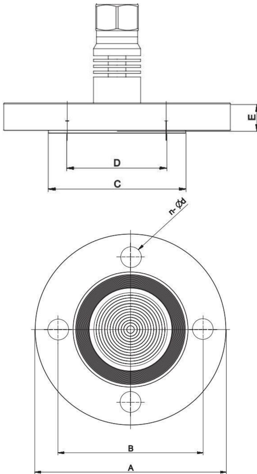
Figure 11.1 Size of diaphragm
