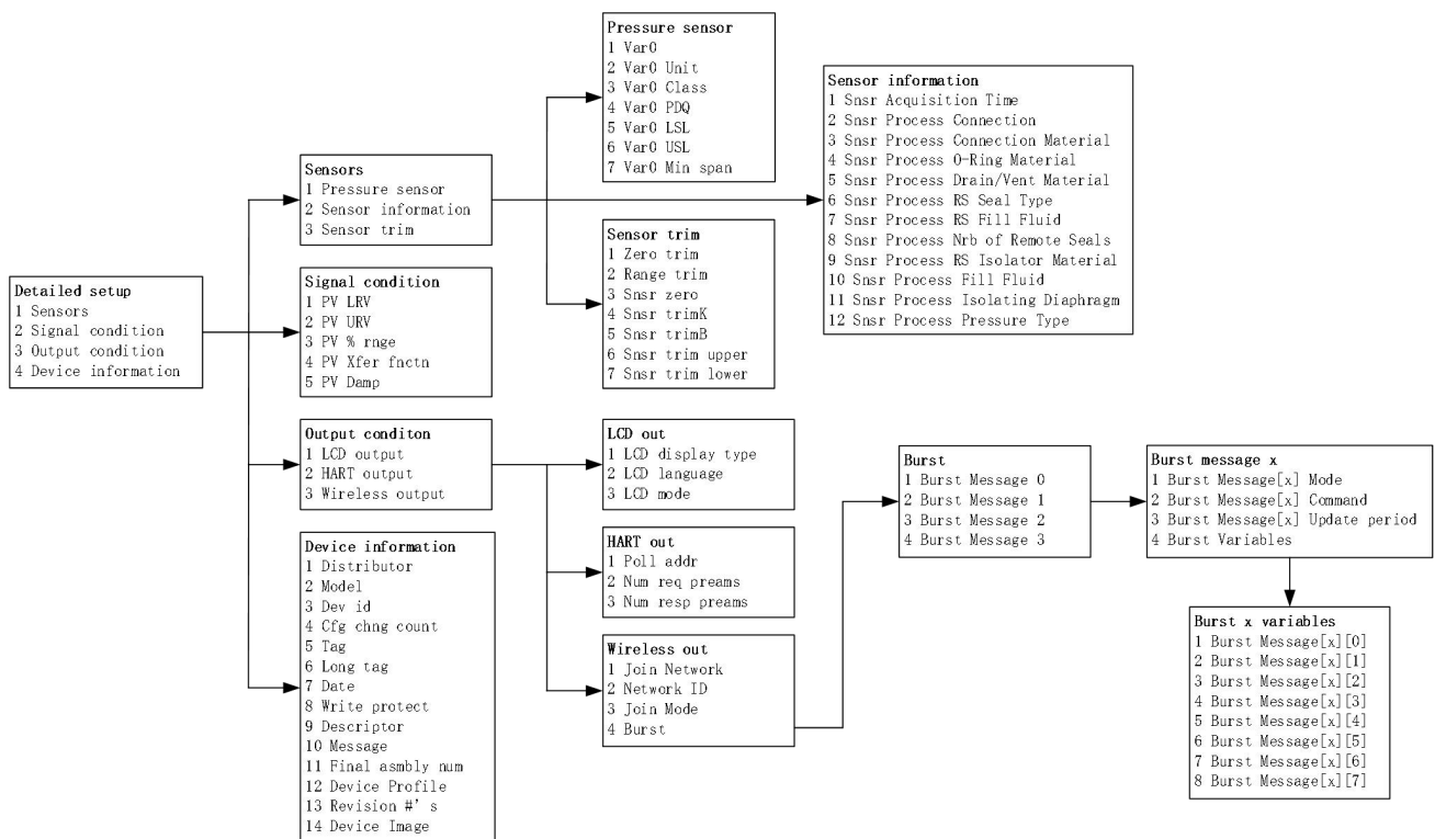
Figure 9.11 DD Menu Tree-details
