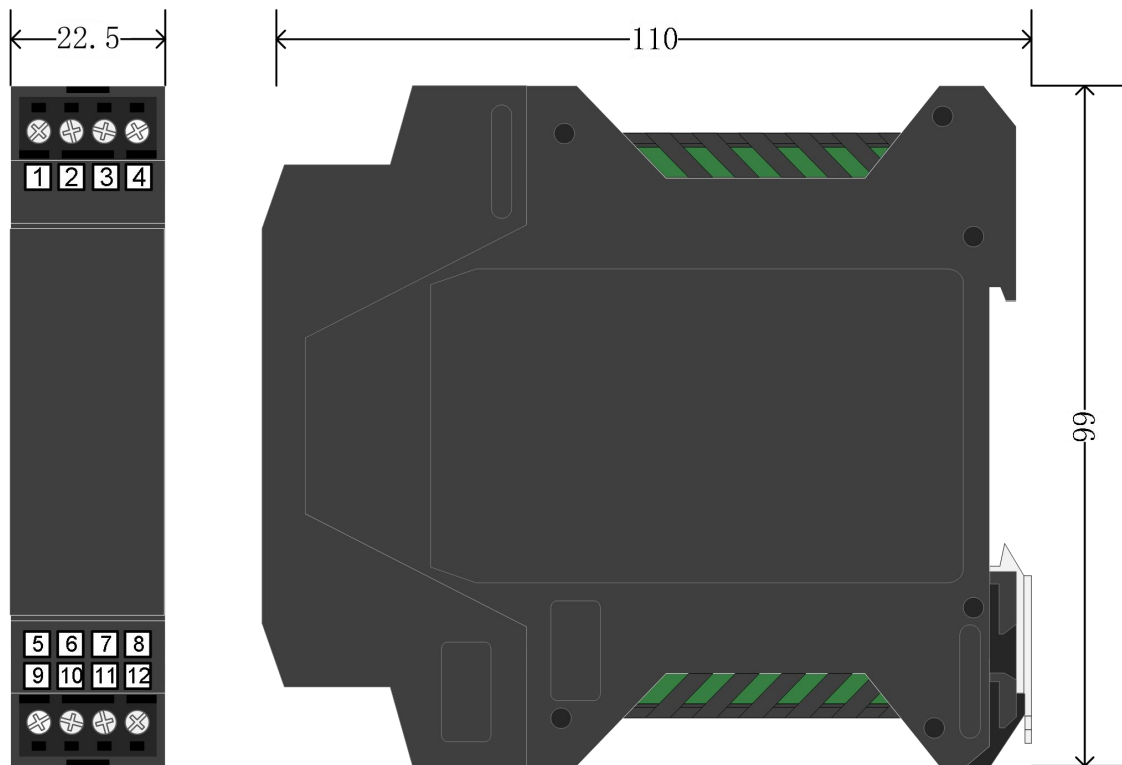
NCS-TT306H-R Rail Installation
