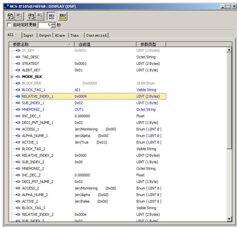
Figure 4.3 LCD Configuration
